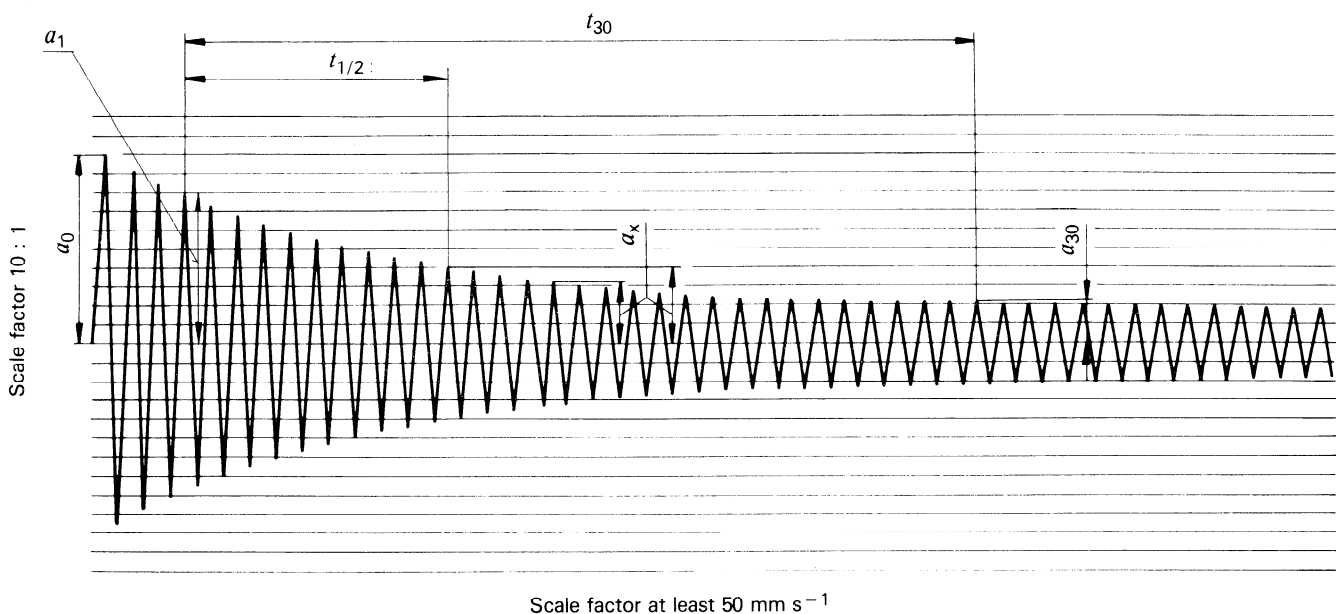
Figure 2 — Typical vibration chart
