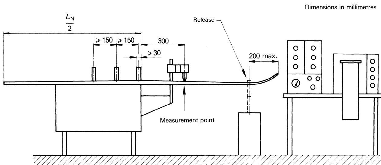
Figure 1 — Test apparatus
