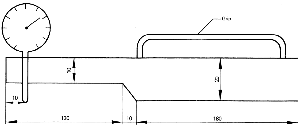
Figure 9 – Measurement of taper depth
