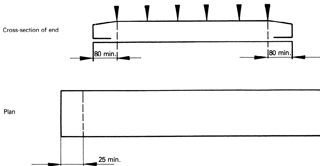
Figure 7 – Measurement of thickness
