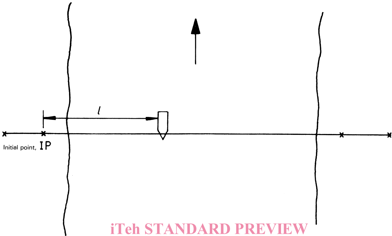
Figure 1 — Position fixing for stream gauging
