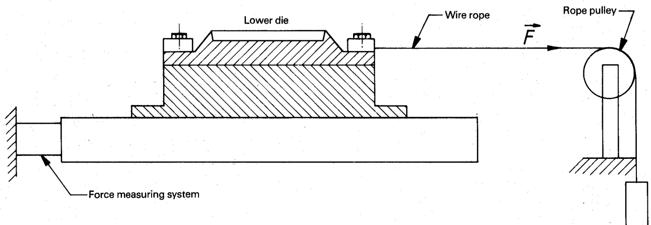
Figure 4 – Calibration equipment for linear shear curemeter
