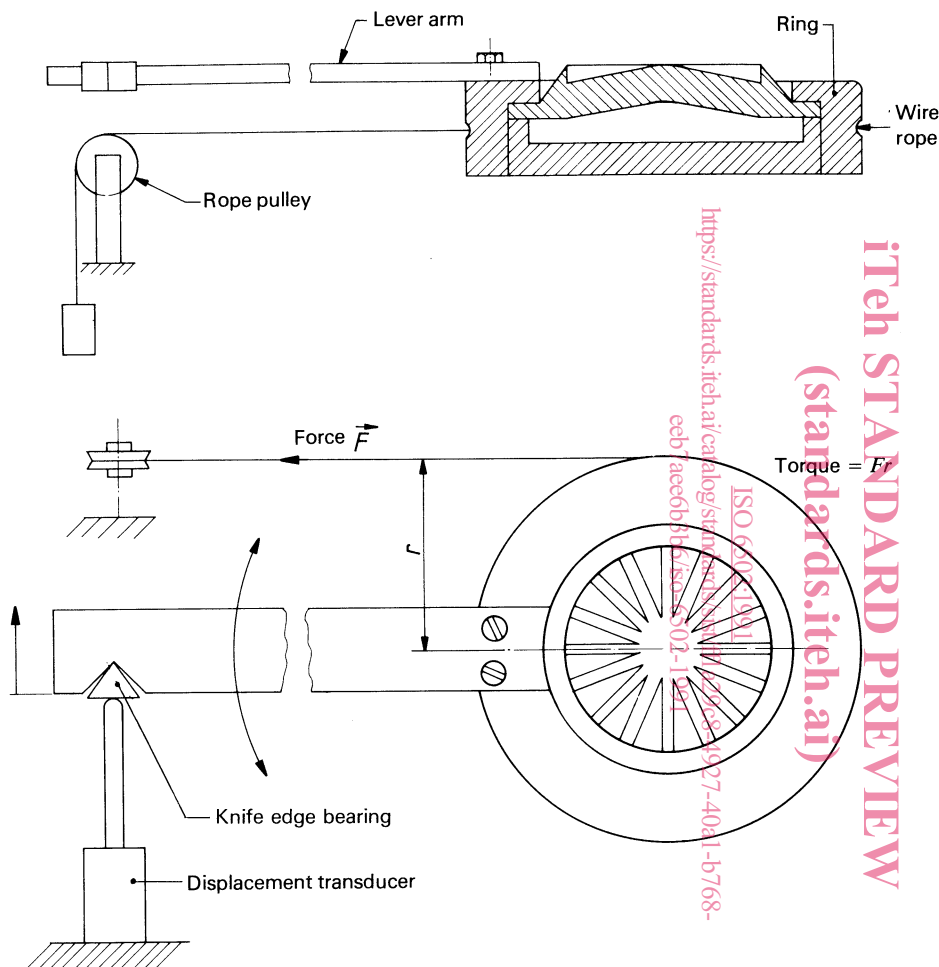
Figure 5 — Calibration equipment for torsion shear curemeter
