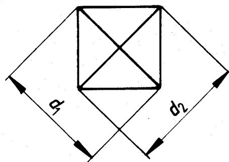
Figure 2 — Empreinte Vickers
