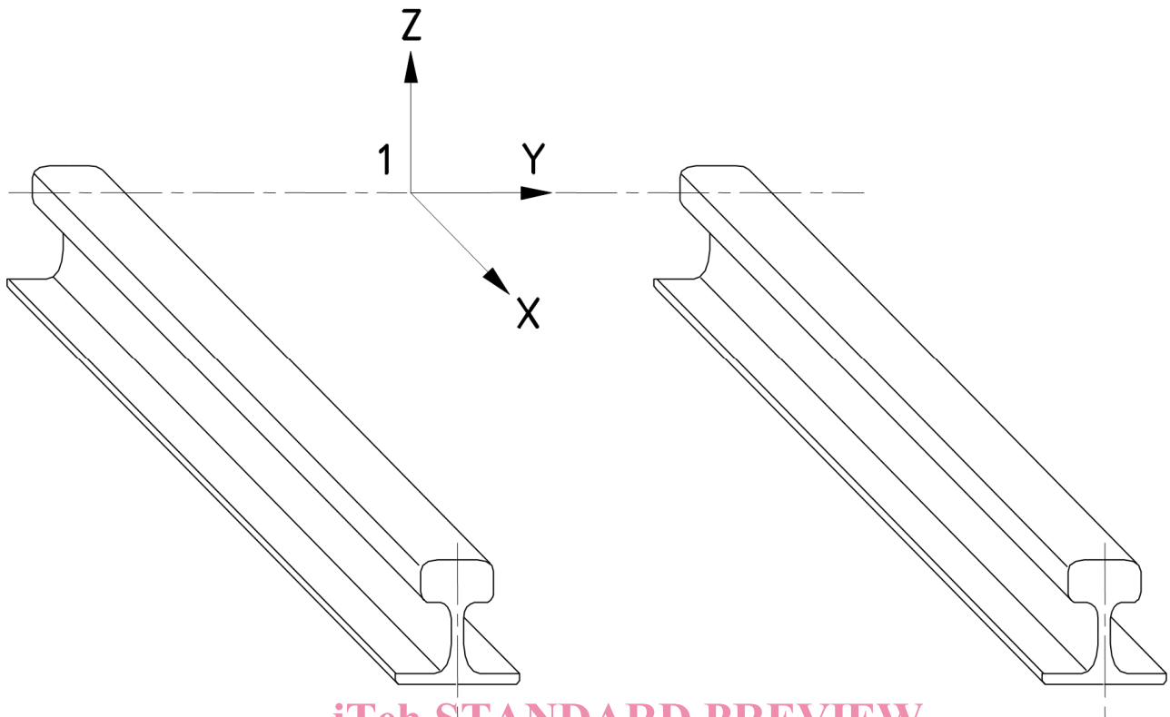
Figure 1 — Track Coordinates
