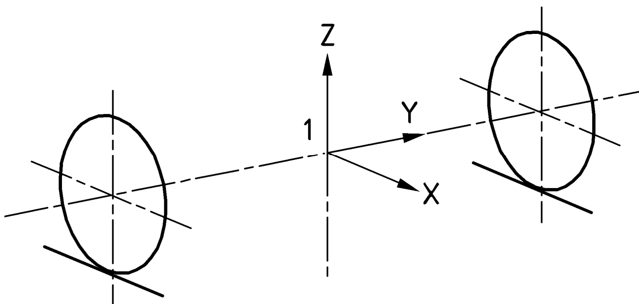
Figure 2 — Rolling Stock Coordinates
