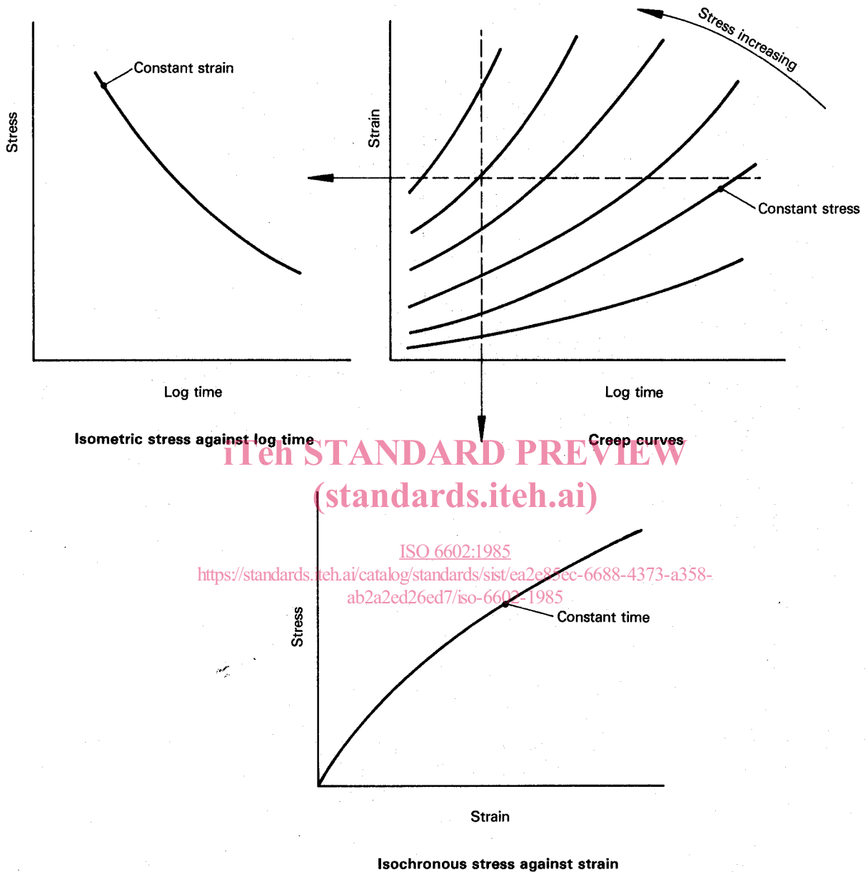
Figure 2 — Creep data — Three methods of presentation
