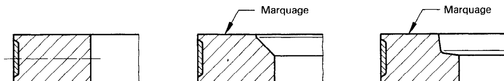
Figure 7 – Segments du type R incrustés
