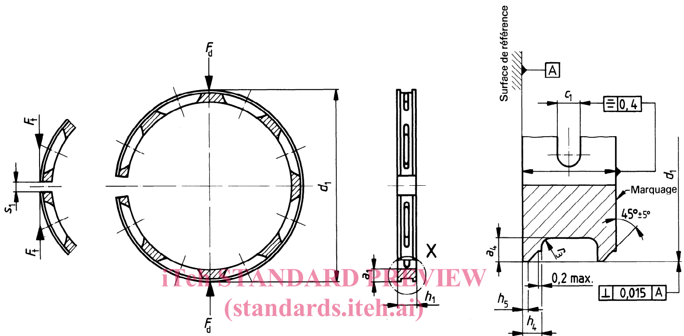
ISO 6625:1986 https://standards.iteh.ai/catalog/standards/sist/45361346-e77e-484f-955a-338080c4b059/iso-6625-1986 Figure 2 – Type G
