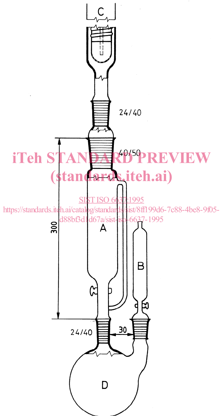
Figure 1 — Decomposition apparatus
