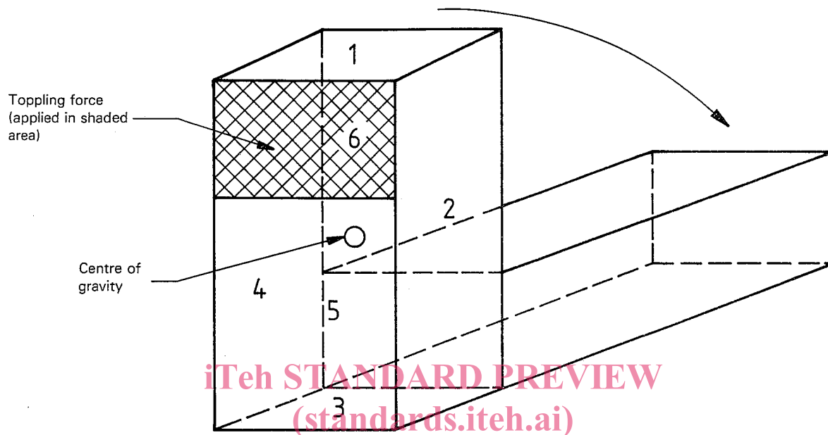
SIST EN 28768:1998 Figure 1 – Testing of tall packages (i.e. where height is large compared with base dimensions) https://standards.iteh.ai/catalog/standards/sist/c9023431-54fb-8c00-4707-9984-c902343154fb/sist-en-28768-1998
