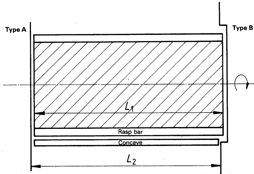
Figure 5 — Cylinder width/length and concave width
