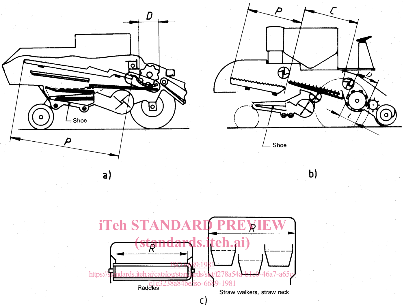
Figure 7 — Walker, riddle and rack dimensions
