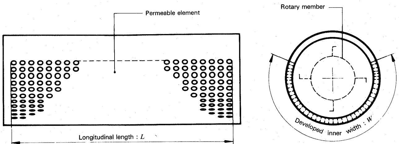
Figure 8 — Dimensions of rotary separator
