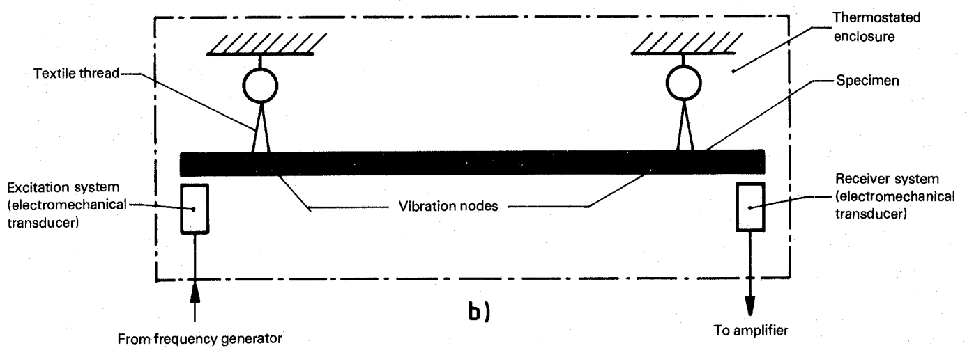
Figure — Schematic diagram of the test apparatus
