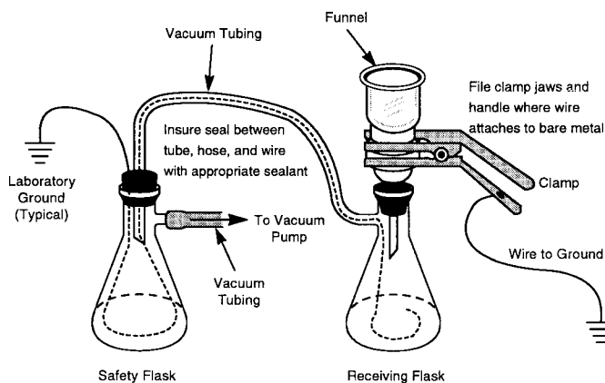
FIG. 1 Schematic of Filtration System
