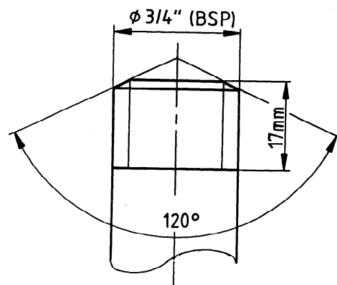
Figure 4 — Mandrel for coupling-nut test
