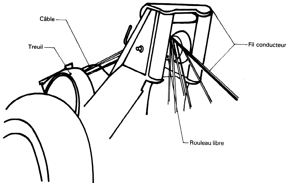
Figure 4 — Treuil fixe
