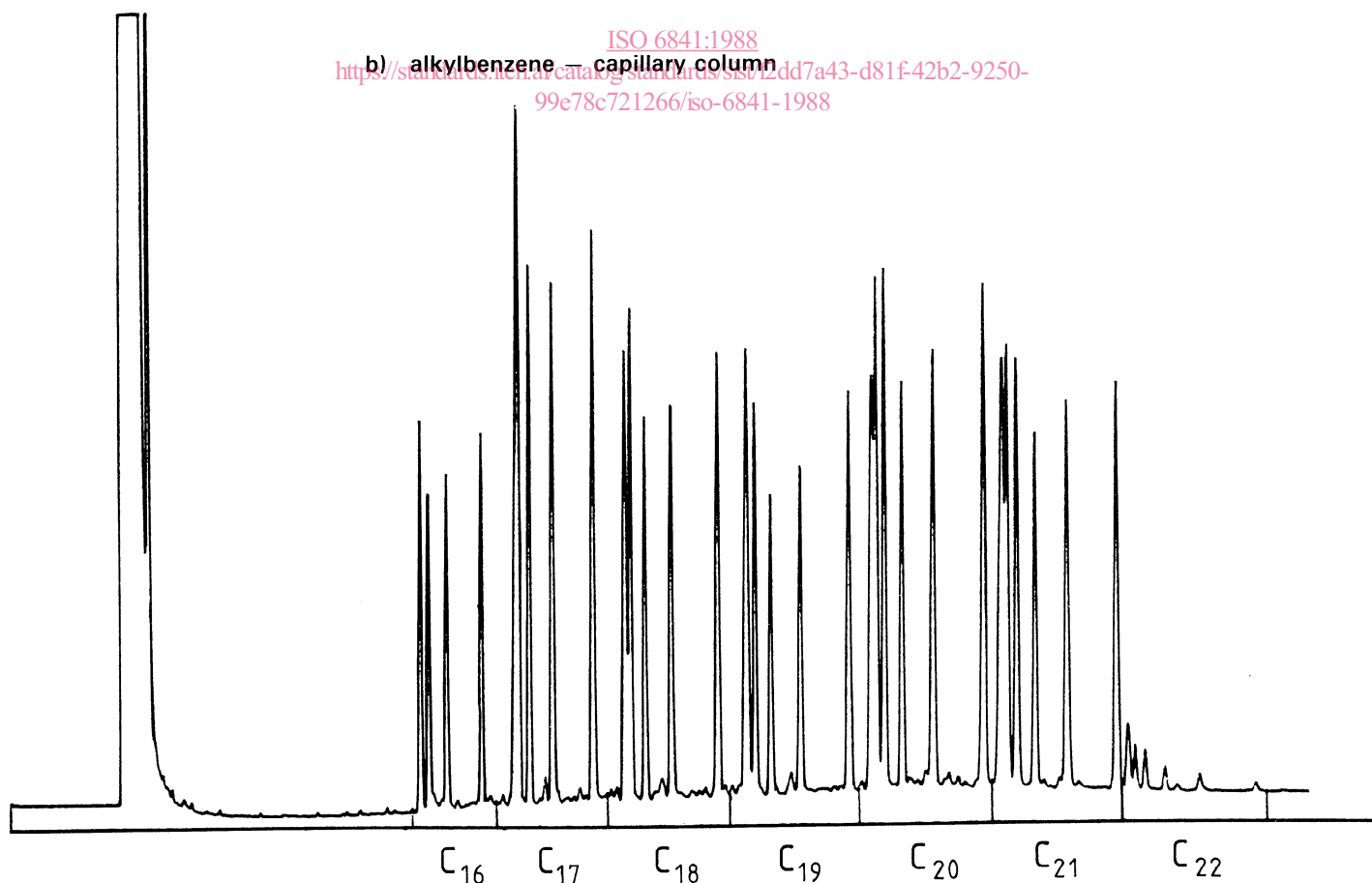
Figure 3 — Typical chromatograms
