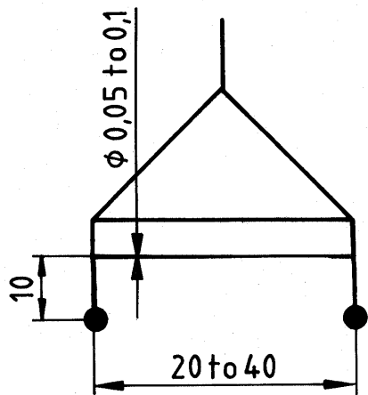
Figure 1 – Stirrup [5.2 a)]
