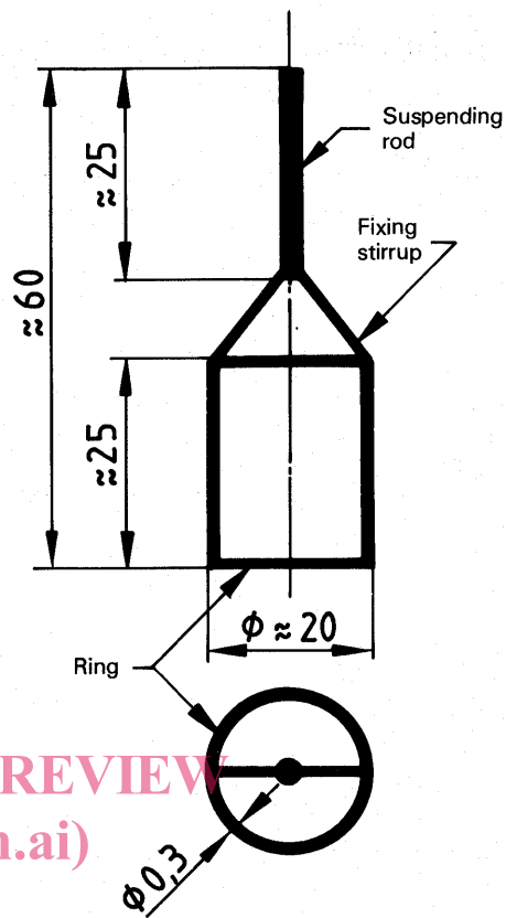
Figure 2 – Ring [5.2 b)]
