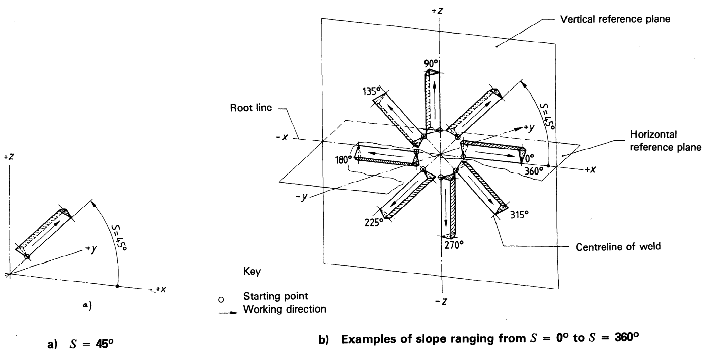
Figure 1 — Slope, S
