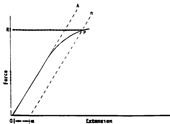
Om = Specified Offset FIG. 1 Force-Extension Curve for Determination of Yield Strength by the Offset Method
