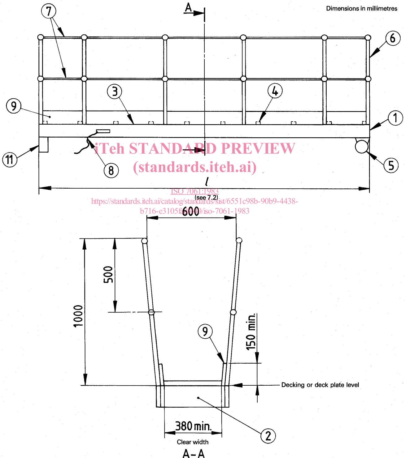
Figure 2 — General arrangement of Type B gangway (for item numbers, see the table)
