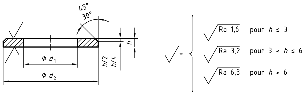
Figure 1 — Dimensions
