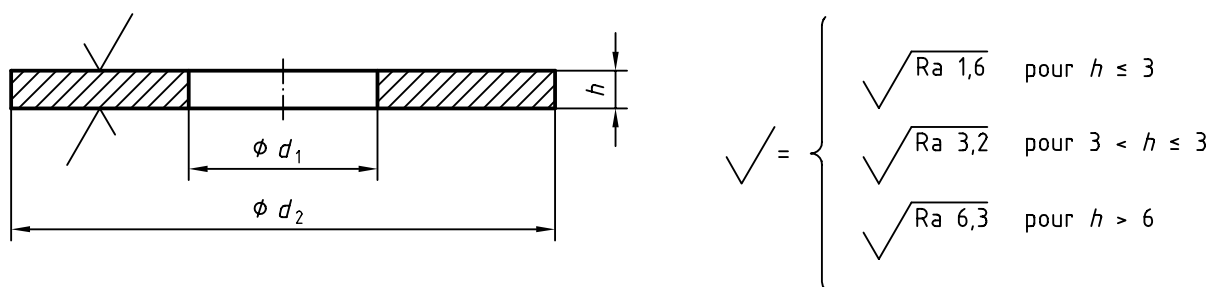
Figure 1 — Dimensions
