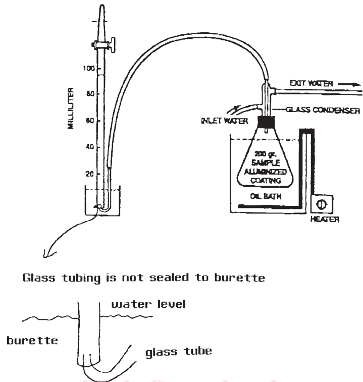
FIG. 1 Hydrogen Gas Generation Test Apparatus
