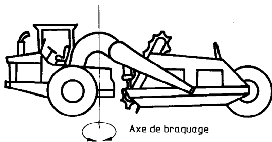
Figure 11 — Direction articulée
