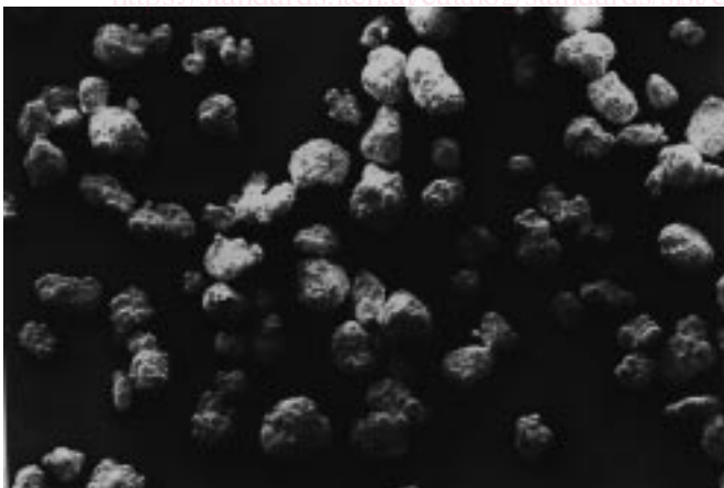
FIG. X2.3 Spherical or Spheroidal—Rough
