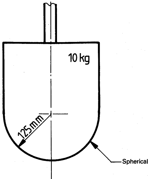
Figure 2 — Bottom impactor
