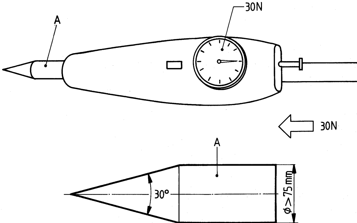
Figure 1 — Example of measuring cone iTeh STANDARD PREVIEW (standards.iteh.ai)
