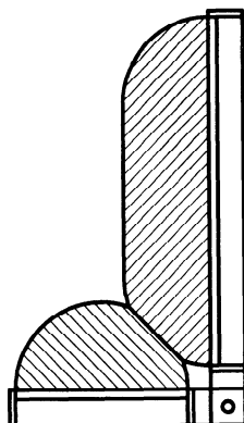
Figure 2 — Vertical section through test rig assembly for foam specimens (see also figures 1 and 2 of ISO 8191-1)
