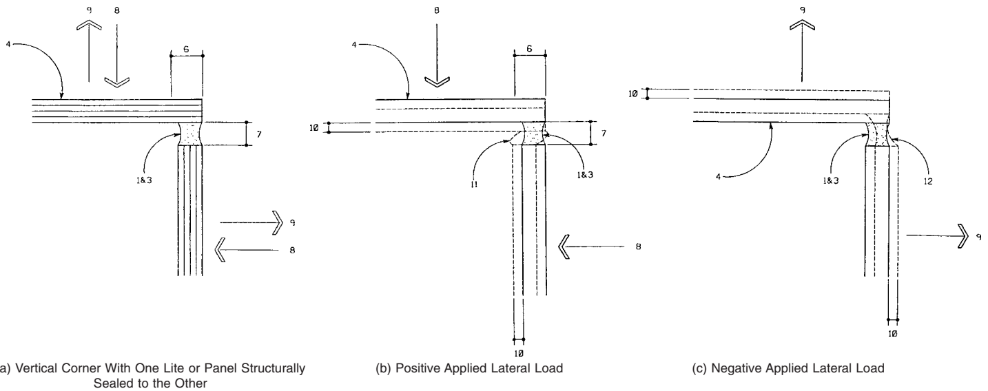
FIG. 2 Applied Load Transfer at a Vertical Corner Structural Sealant Joint (see Fig. 1 for Legend)
