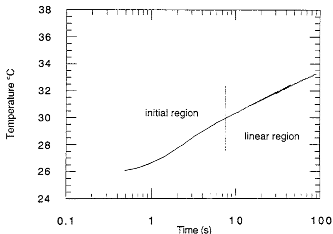
FIG. 1 Line-Source Transient
