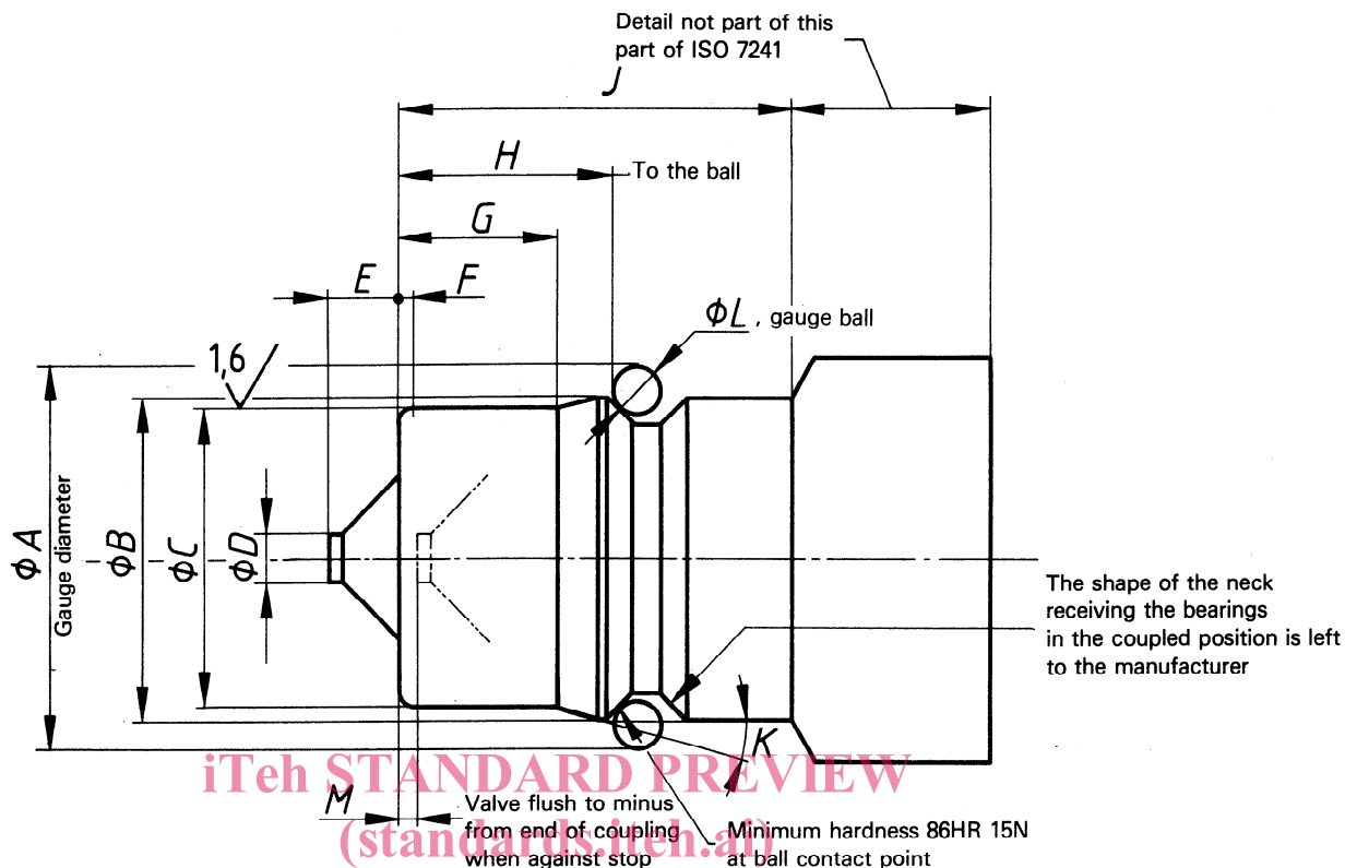
ISO 7241-1:1987 https://standards.iteh.ai/catalog/standards/sist/3b30557a-8bee-4738-afa6-c760c1768187/iso-7241-1-1987 Figure 2 – Dimensional requirements, series "B" – Sizes 5 to 25
