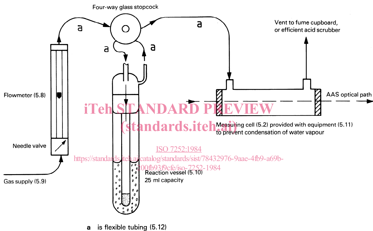
Figure 2 – Typical apparatus for the determination of mercury by flameless atomic absorption spectrometry
