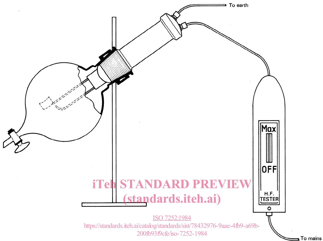
Figure 3 – General view of combustion apparatus
