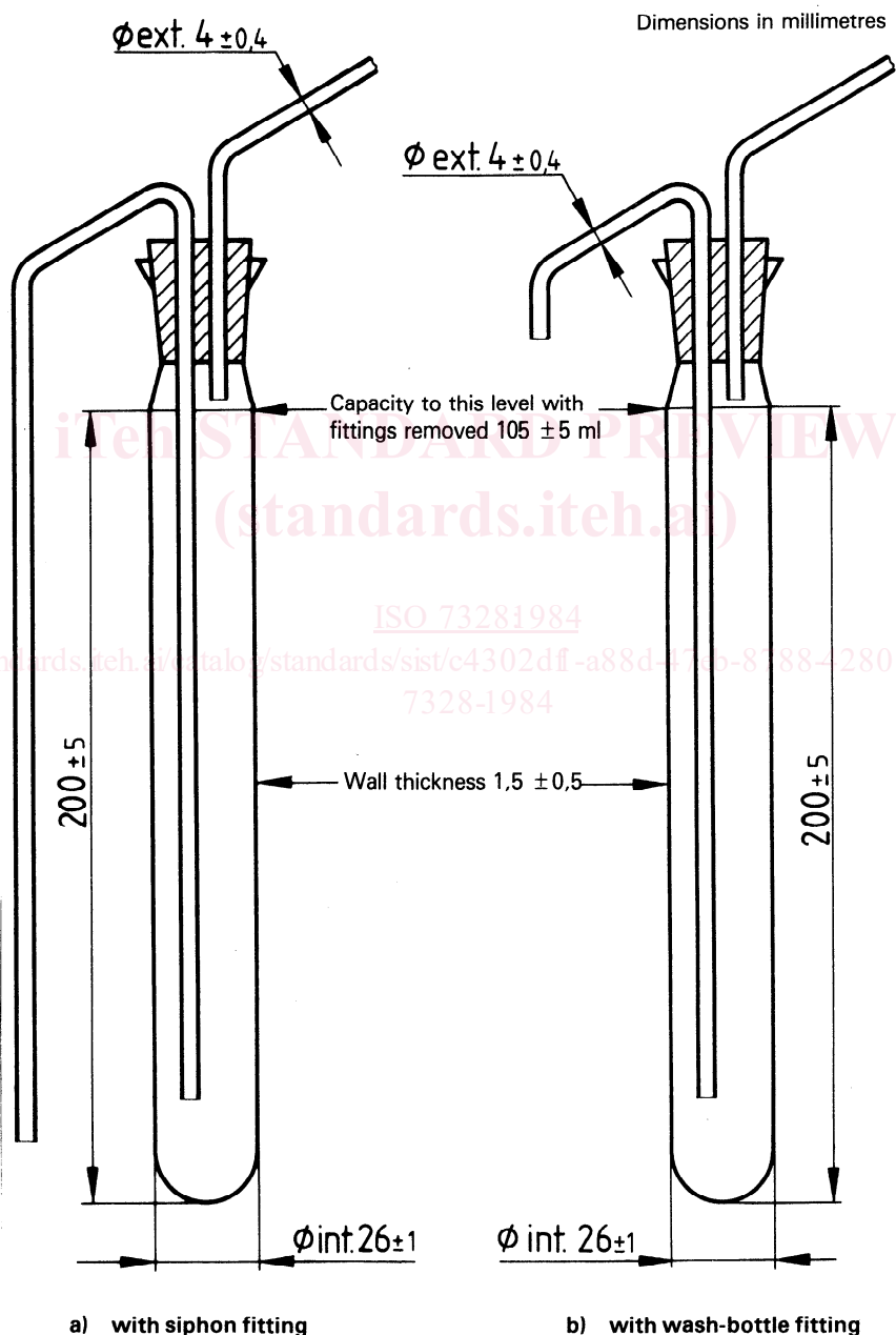
Figure 3 — Examples of extraction tubes
