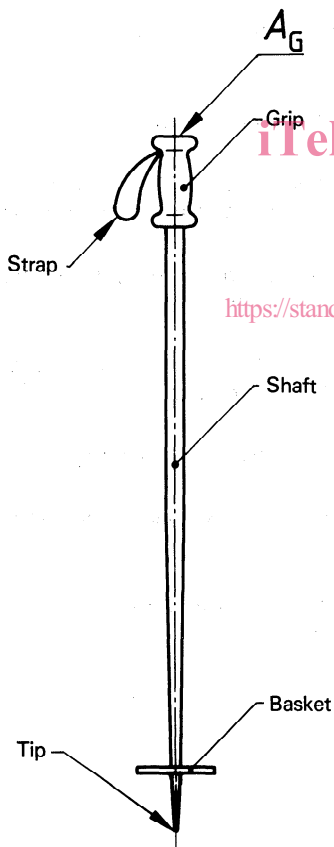
Figure 1 — Ski-pole — Terms
