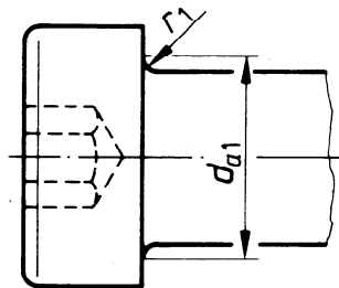
Alternative form at head/shank junction permissible
