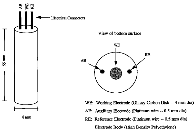
FIG. 1 Combination Electrode
