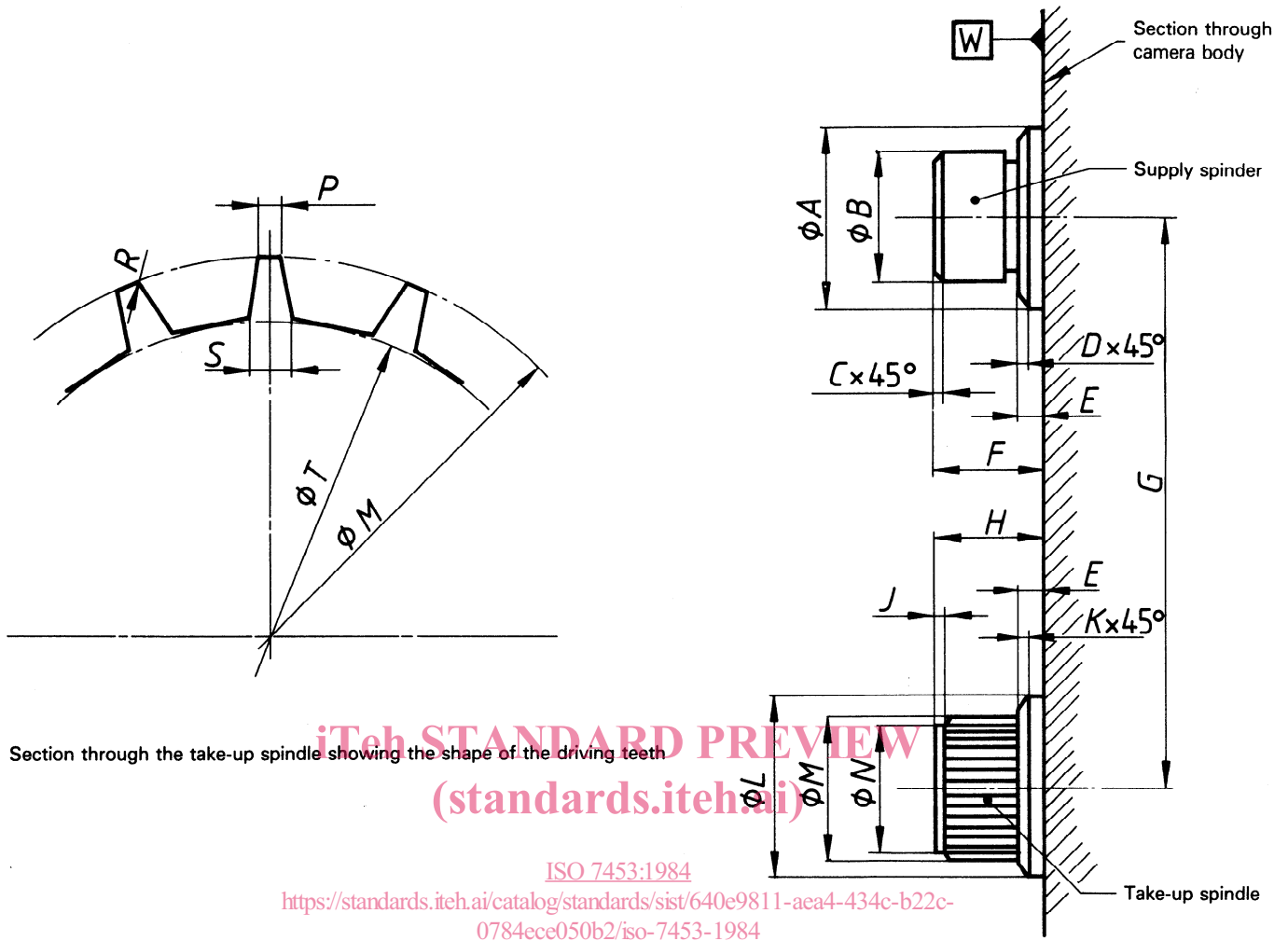
Figure 3 — Camera spindle dimensions and specifications
