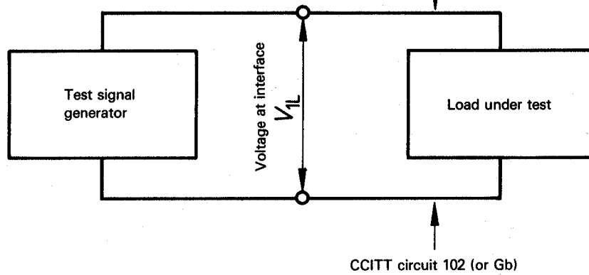
Figure 2 — Test arrangement for V.28 loads
