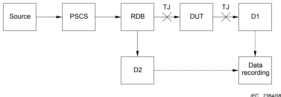
Figure 2 – Measurement apparatus
