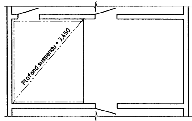
Figure 8 — Plafond suspendu
