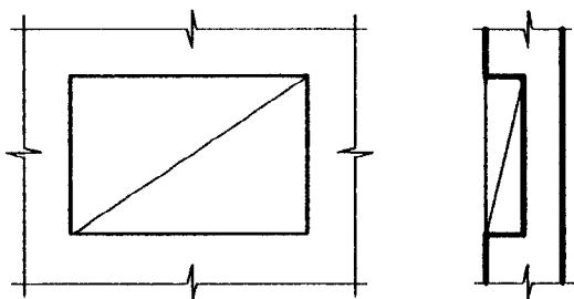
Figure 10 — Retraits
