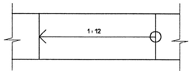
Figure 5 — Ramp
