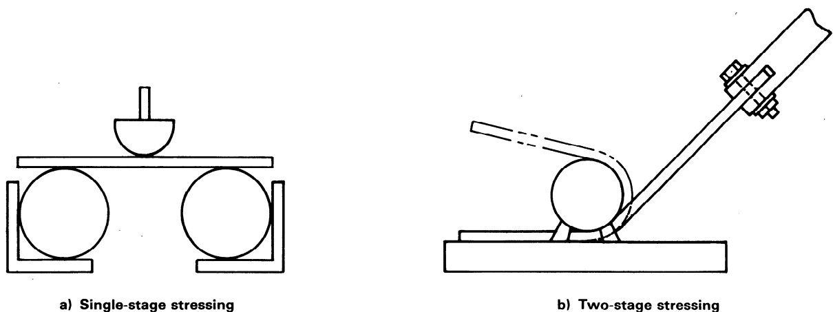
Figure 2 — Methods of stressing U-bend specimens
