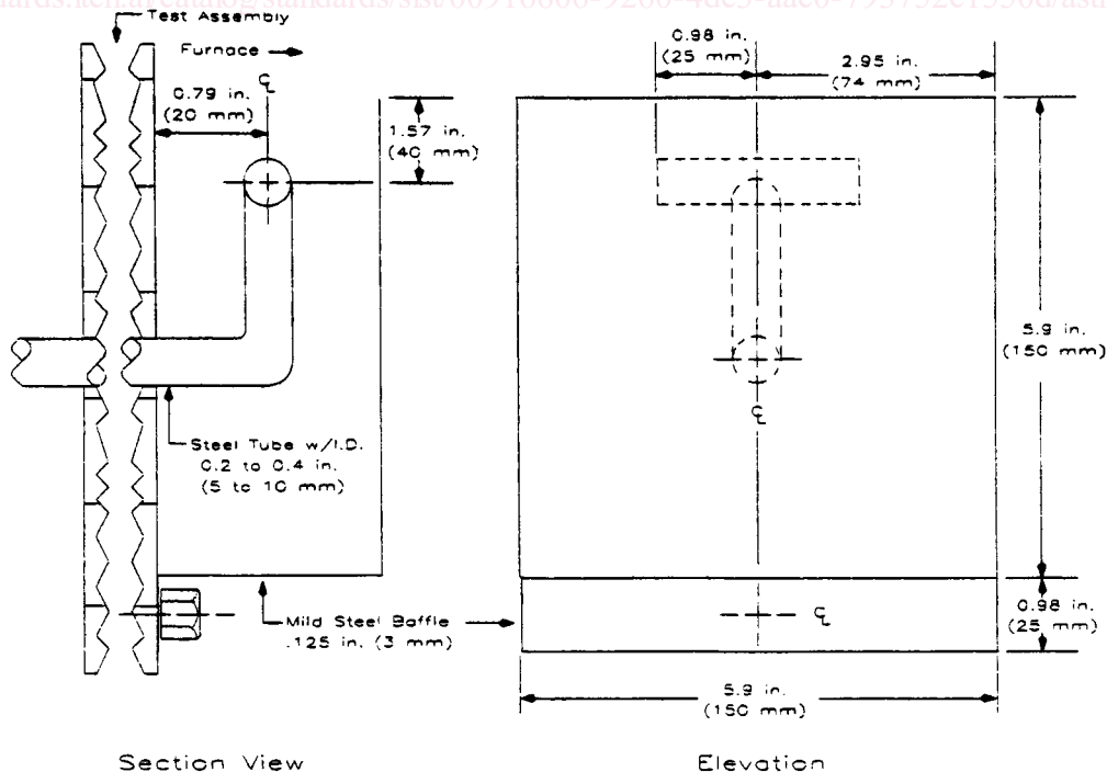
FIG. 3 T-Shaped Sensor
