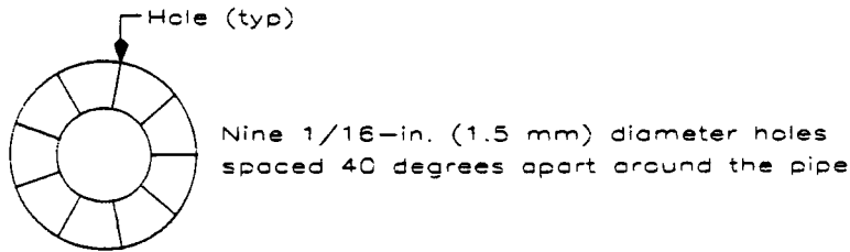
Enlarged Section View A - A
