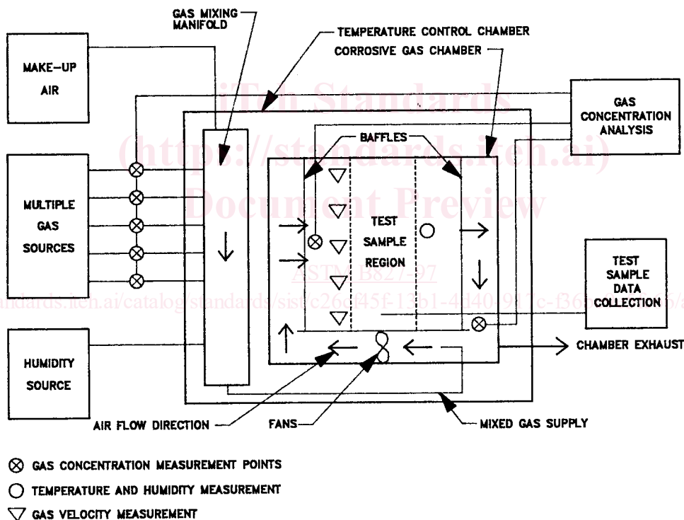
FIG. 3 Schematic Horizontal Recirculating Mixed Flowing Gas (MFG) Test System
