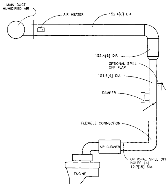
NOTE 1—Dimensions are in millimetres and (inches). FIG. 2 Typical Test Stand Intake Air Supply System
