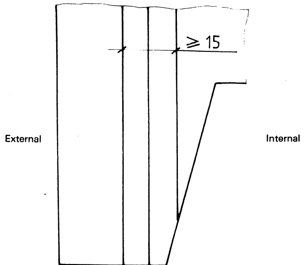
Figure 3 – Vertical section of vertical joint
