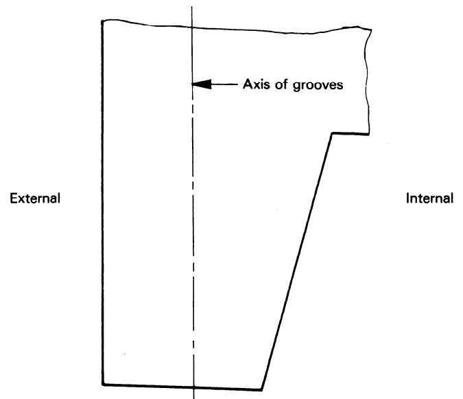
Figure 5 – Vertical section of vertical joint
