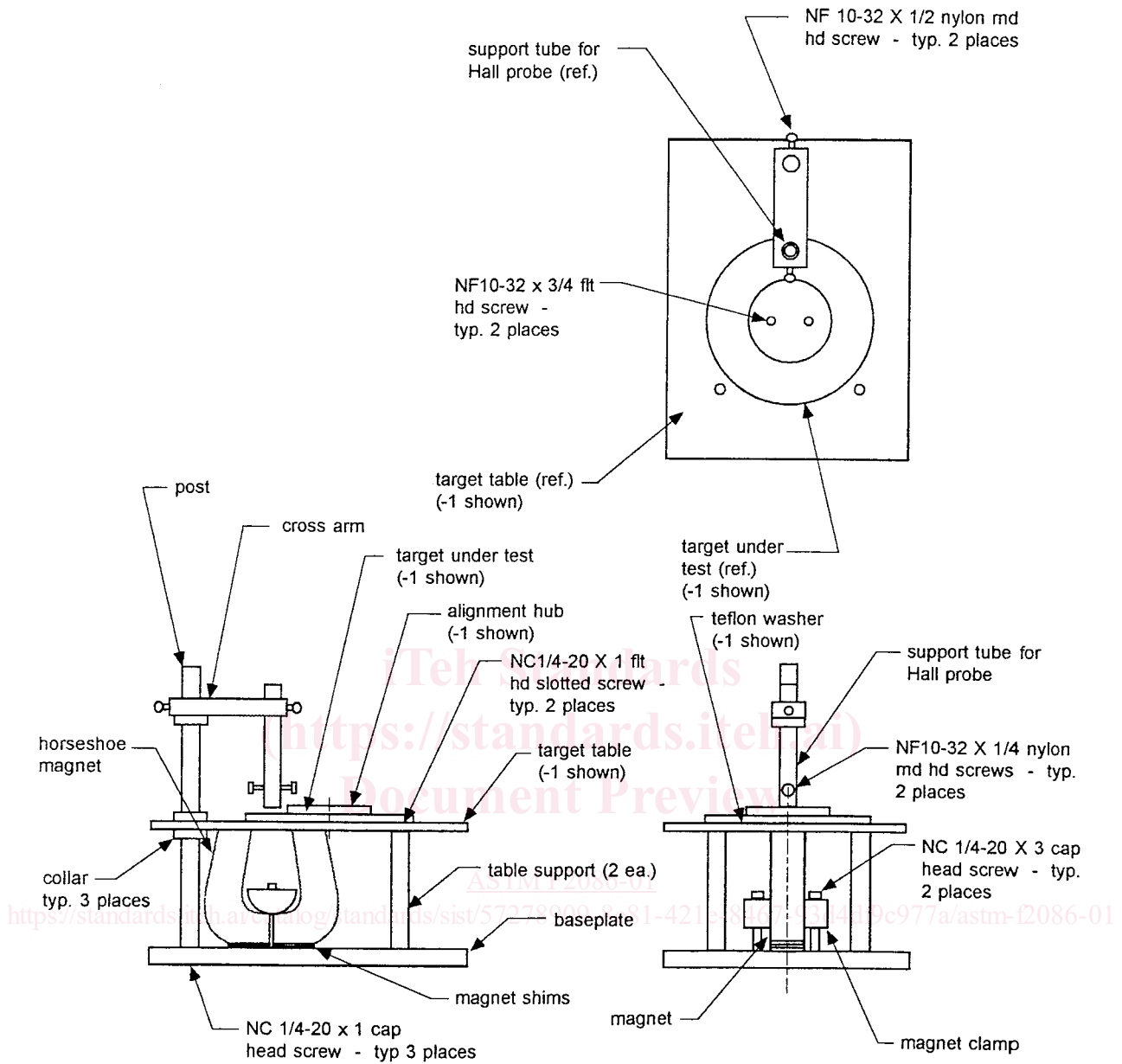
FIG. X1.1 Magnetic Test Fixture - Assy
