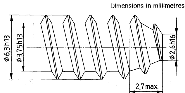
Figure 1 — Thread and end configuration
