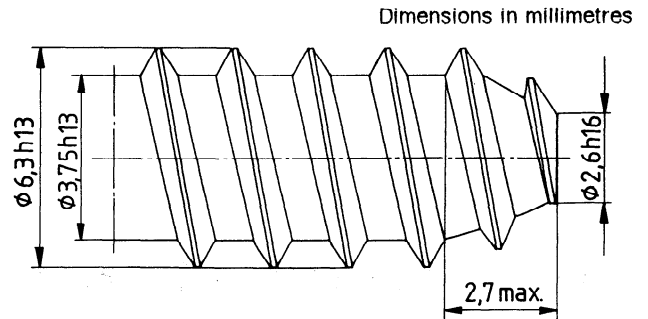
Figure 1 — Thread and end configuration
